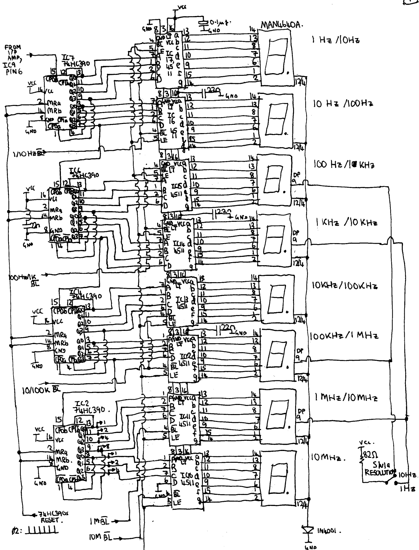
RADIO FREQUENCY COUNTER. HANS SUMMERS, 1993
